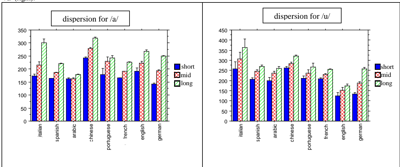
Figures 14-15: Distance (dispersion) from acoustic center for each language for all duration categories for vowel /a/ (left) and vowel /u/ (right).
