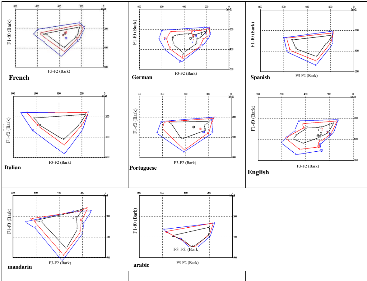
Figure 6 - 13: mean average values of f1-f0 and f3-f2 for all languages according to their duration. From inside to outside (black [30 – 50ms], red [60 - 80], blue [90 - 110]). Male and female results are merged.
