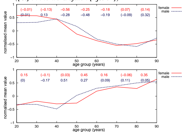
Figure 4: Normalised tendencies (separately for each gender) for mean F_1 (top) and mean F_2 (bottom) ([ɛ:] in the word själen [ˈʃjɛ:lɛn]).
