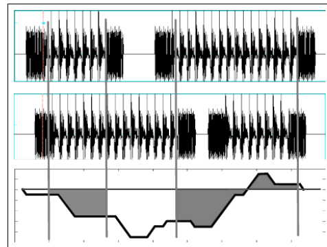
Figure 1: Quantification of asynchrony between two stylized utterances. The warp path obtained by dynamic time warping has been replotted as a function of (referent) time at the bottom. Portions of the area under the curve corresponding to voiced portions of the referent (top waveform) are summed.
